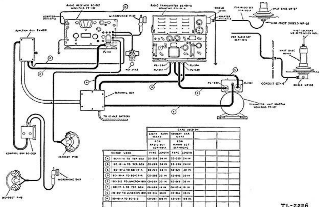
FIGURE 12.—Radio sets SCR-193-A and SCR-193-C, cording diagram.
