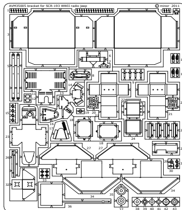
AVM35005 bracket
